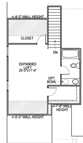
SECOND FLOOR STANDARD
