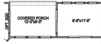
3 SEASON ROOM
