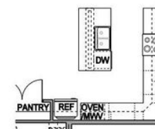
DELUXE KITCHEN
