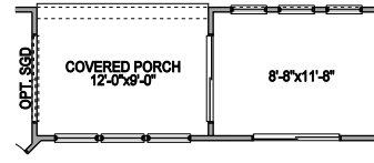
3 SEASON ROOM
