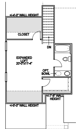
SECOND FLOOR STANDARD
