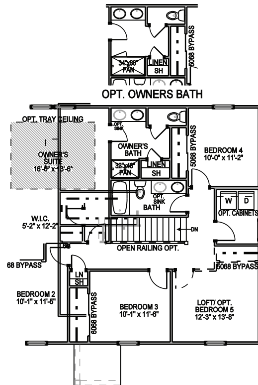
THE HAYES SECOND FLOOR - 1,255 S.F.
